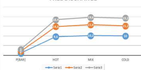
FLOW RATE [L/MIN]-G3/4" FREE DISCHARGE
